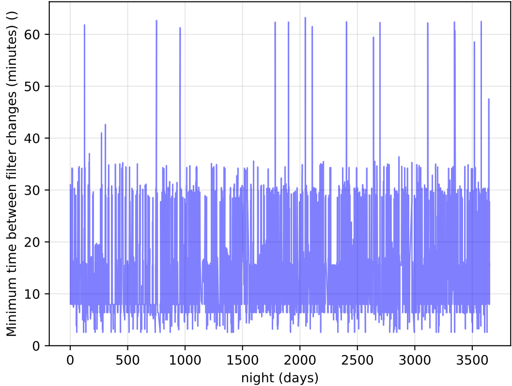
too_elab_r16_d2_gz_v3.4_10yrs Per Night: Minimum time between filter changes (minutes)
