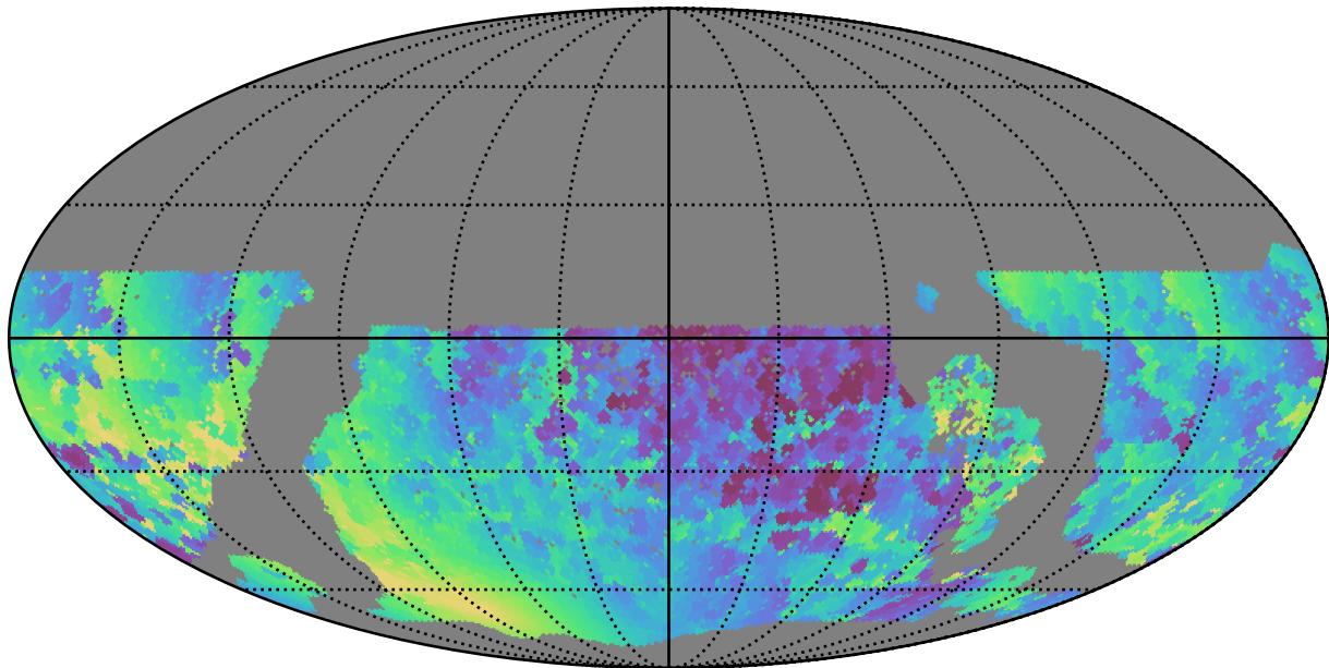
too_elab_r16_d2_gz_v3.4_10yrs WFD y band: Min solarElong
