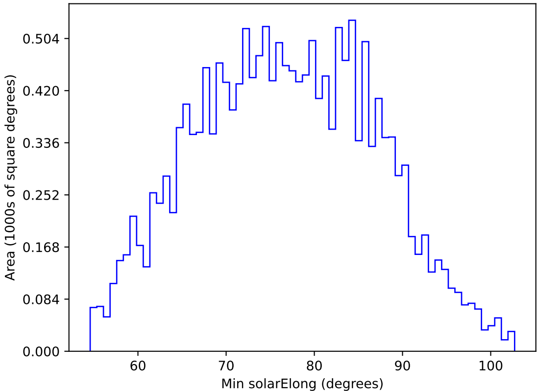
too_elab_r16_d2_gz_v3.4_10yrs WFD u band: Min solarElong
