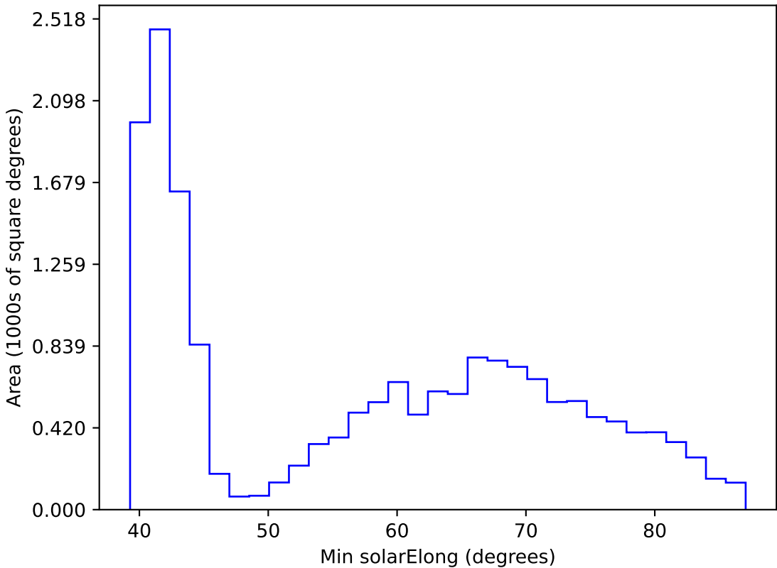
too_elab_r16_d2_gz_v3.4_10yrs WFD r band: Min solarElong
