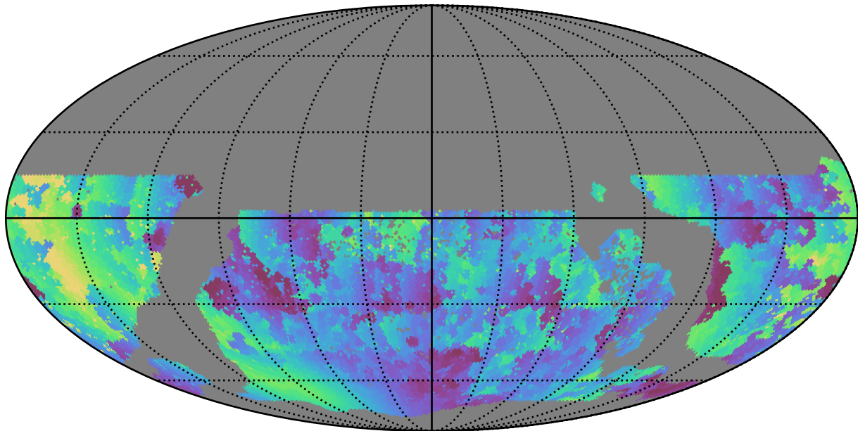
too_elab_r16_d2_gz_v3.4_10yrs WFD g band: Min solarElong
