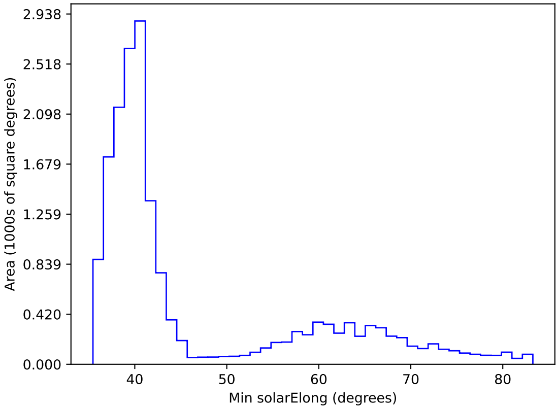
too_elab_r16_d2_gz_v3.4_10yrs WFD all bands: Min solarElong
