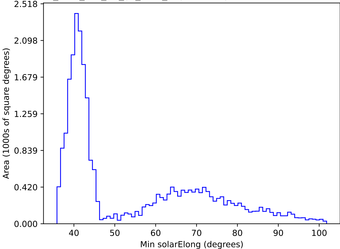
too_elab_r16_d2_gz_v3.4_10yrs All sky z band: Min solarElong
