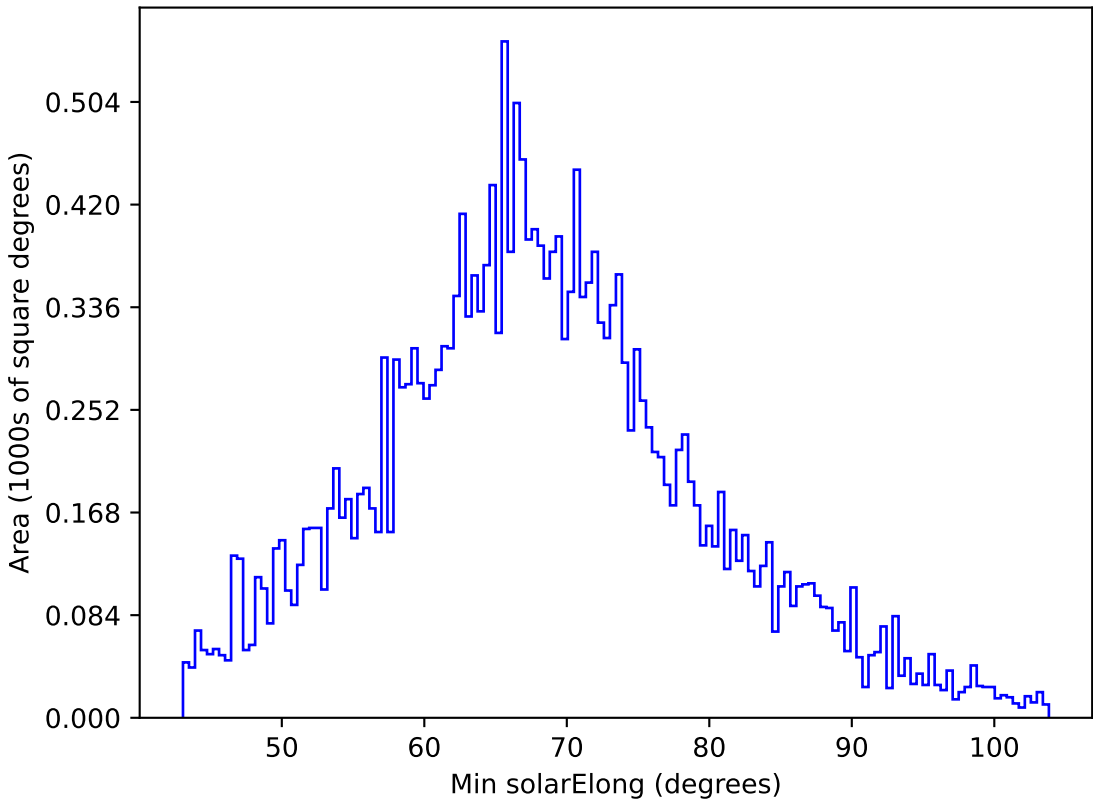
too_elab_r16_d2_gz_v3.4_10yrs All sky y band: Min solarElong
