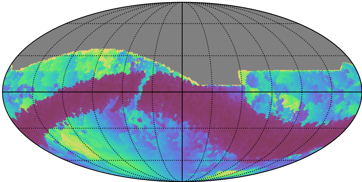
too_elab_r16_d2_gz_v3.4_10yrs All sky r band: Min solarElong
