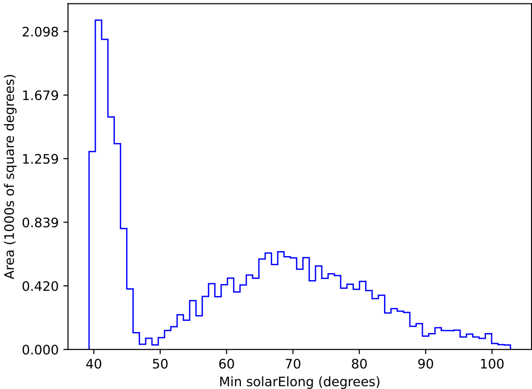
too_elab_r16_d2_gz_v3.4_10yrs All sky r band: Min solarElong
