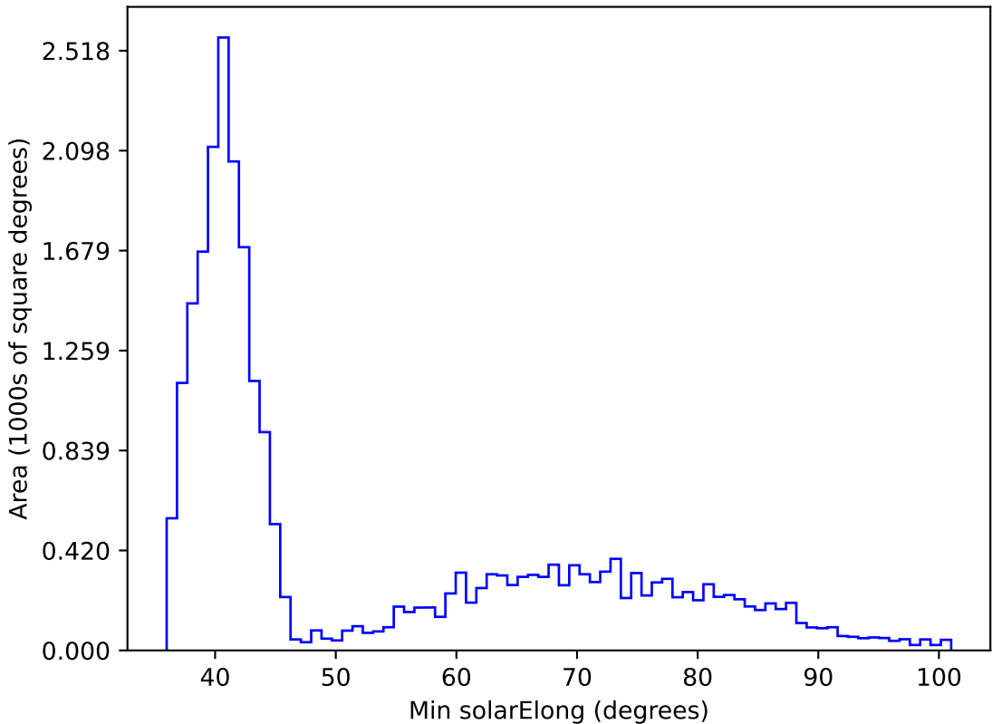
too_elab_r16_d2_gz_v3.4_10yrs All sky i band: Min solarElong
