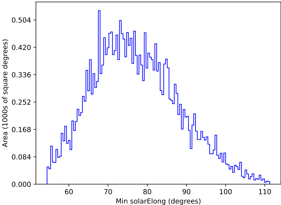
too_elab_r16_d2_gz_v3.4_10yrs All sky g band: Min solarElong
