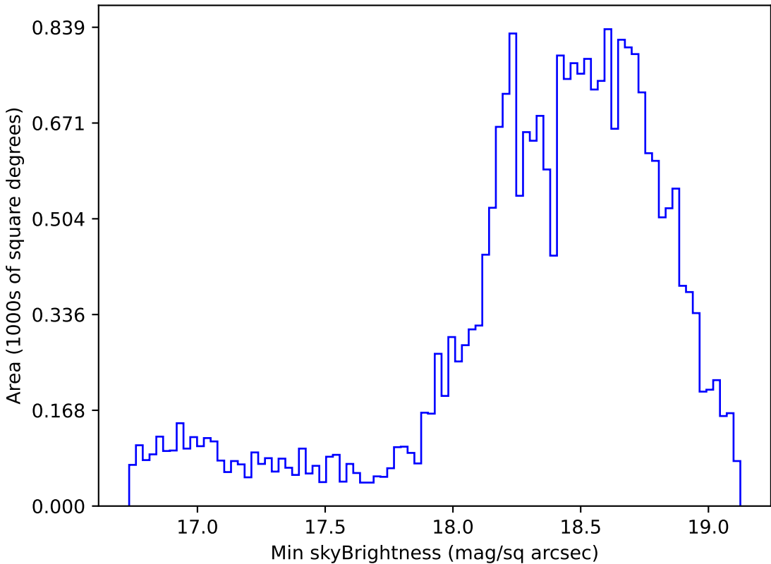
too_elab_r16_d2_gz_v3.4_10yrs Yr 1 z band: Min skyBrightness
