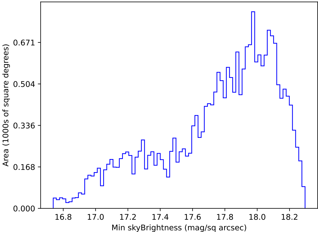
too_elab_r16_d2_gz_v3.4_10yrs Yr 1 y band: Min skyBrightness
