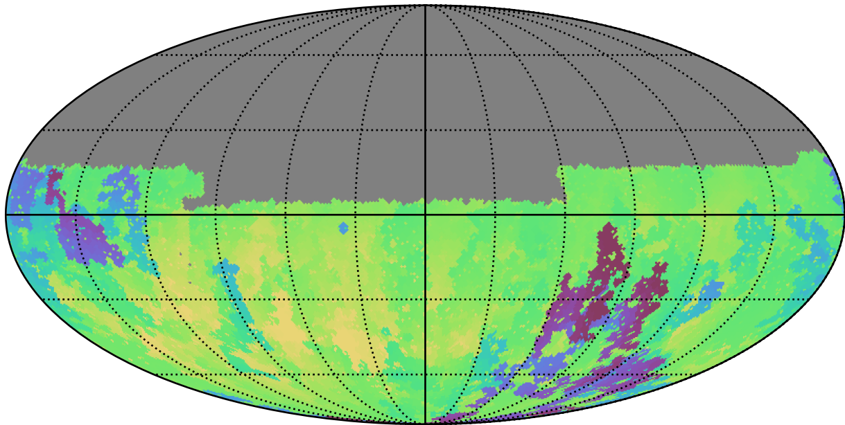
too_elab_r16_d2_gz_v3.4_10yrs Yr 1 u band: Min skyBrightness
