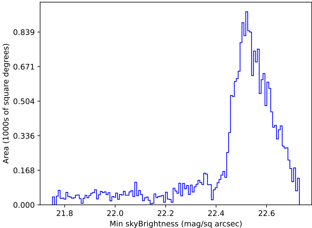
too_elab_r16_d2_gz_v3.4_10yrs Yr 1 u band: Min skyBrightness
