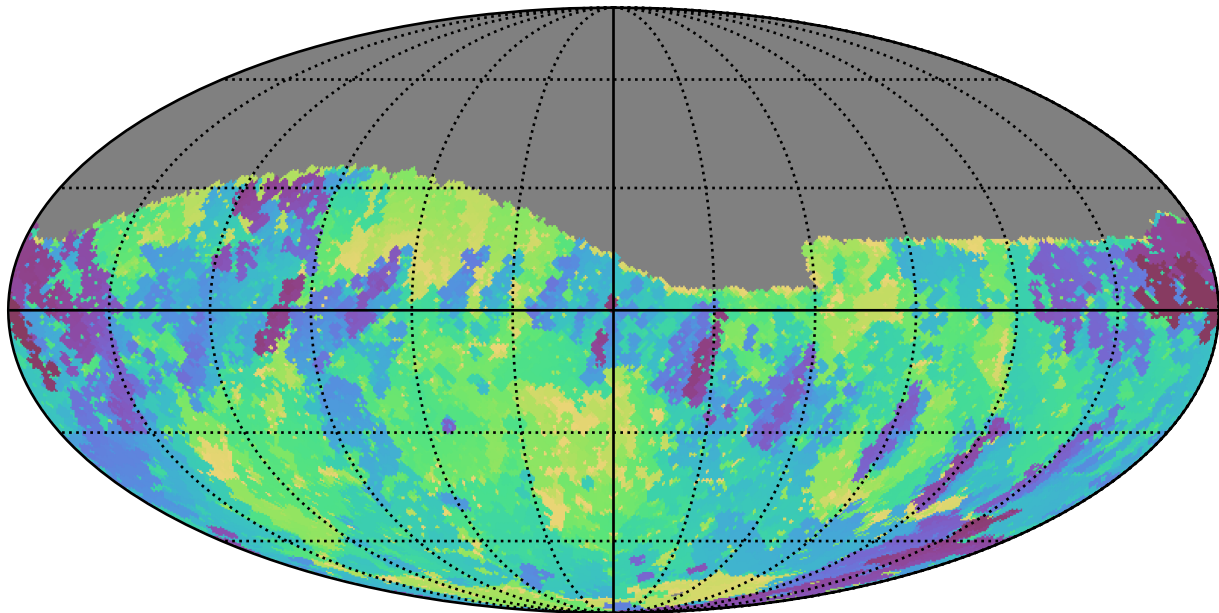
too_elab_r16_d2_gz_v3.4_10yrs Yr 1 r band: Min skyBrightness
