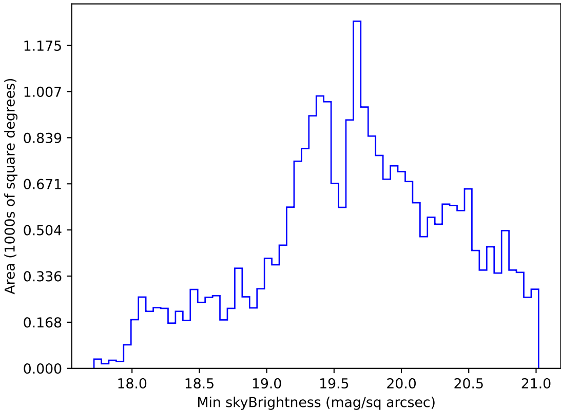
too_elab_r16_d2_gz_v3.4_10yrs Yr 1 r band: Min skyBrightness
