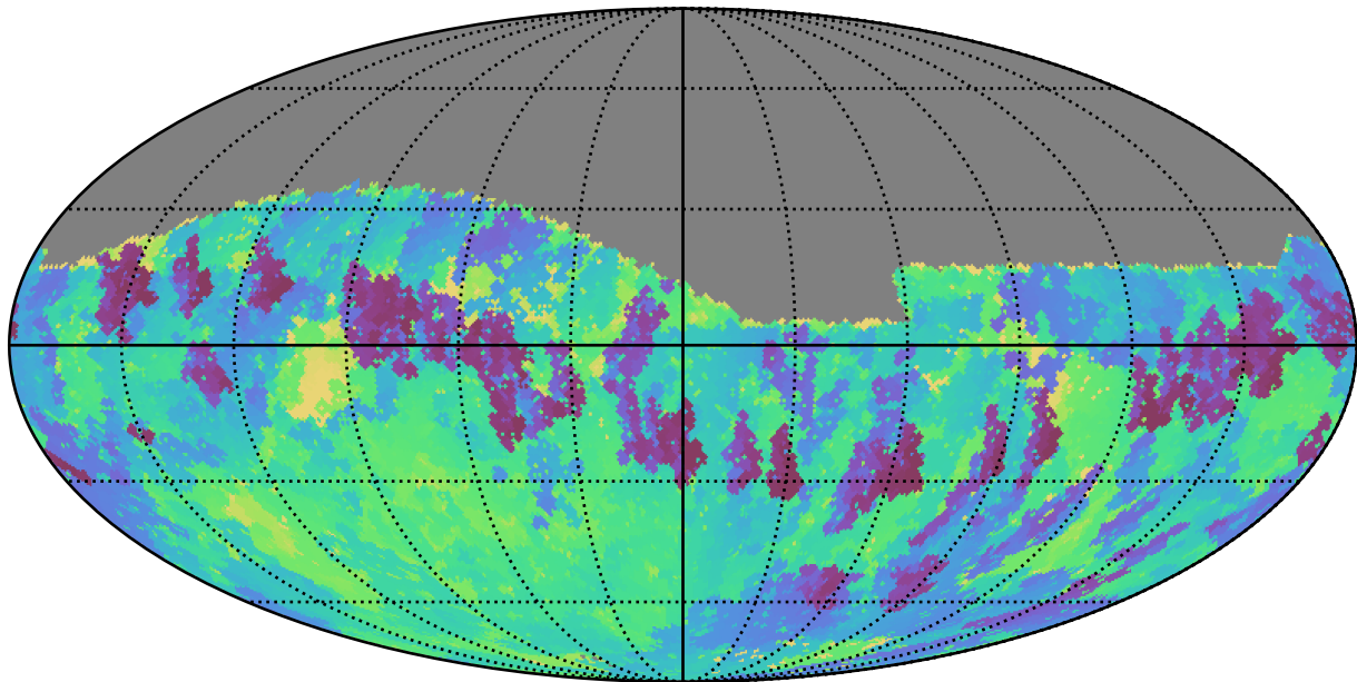
too_elab_r16_d2_gz_v3.4_10yrs Yr 1 i band: Min skyBrightness
