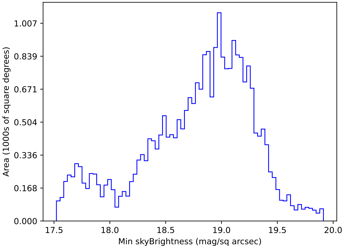
too_elab_r16_d2_gz_v3.4_10yrs Yr 1 i band: Min skyBrightness
