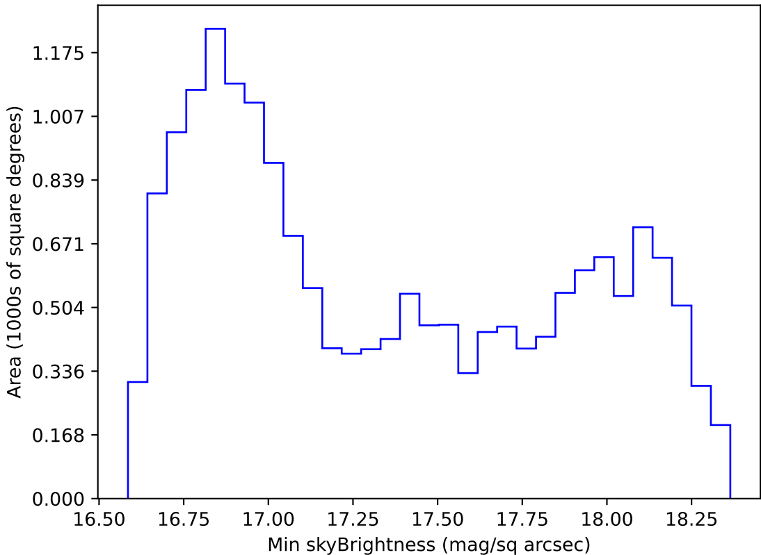
too_elab_r16_d2_gz_v3.4_10yrs WFD z band: Min skyBrightness
