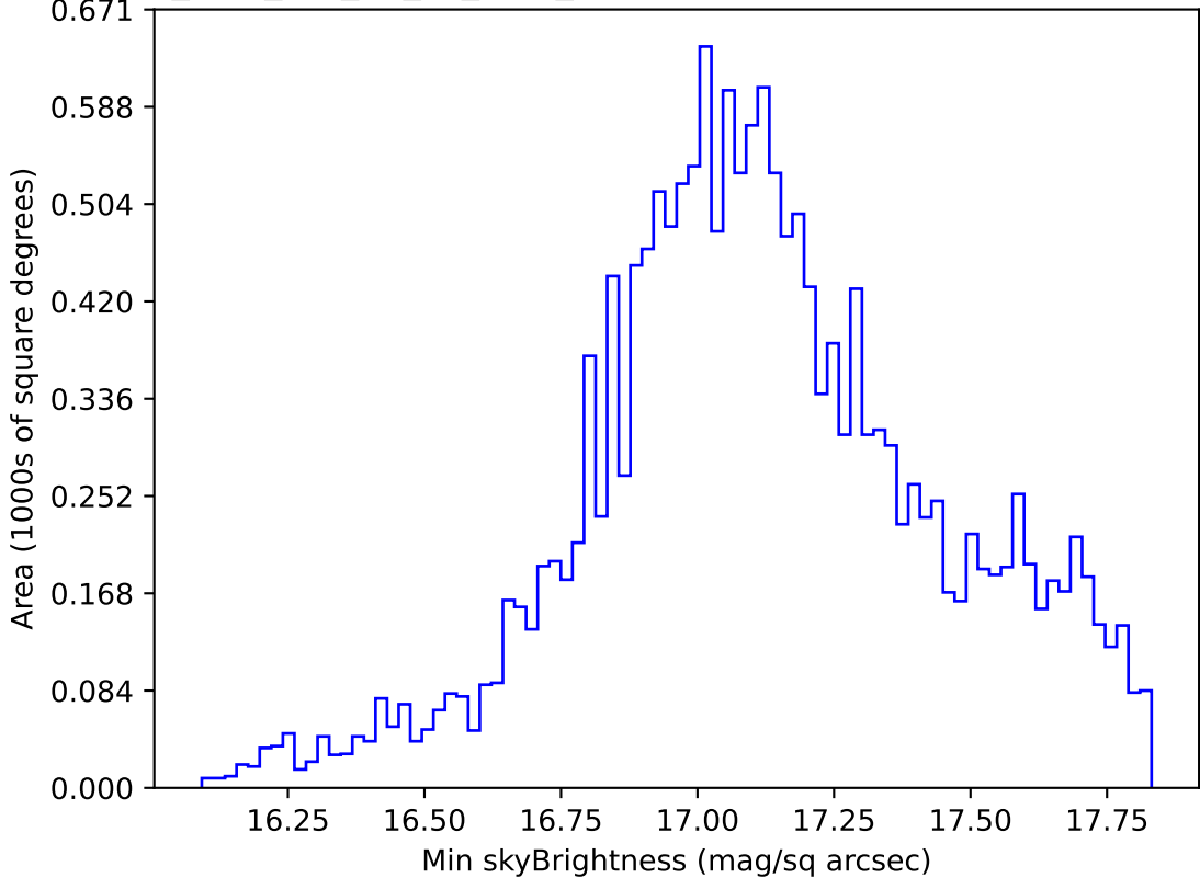
too_elab_r16_d2_gz_v3.4_10yrs WFD y band: Min skyBrightness
