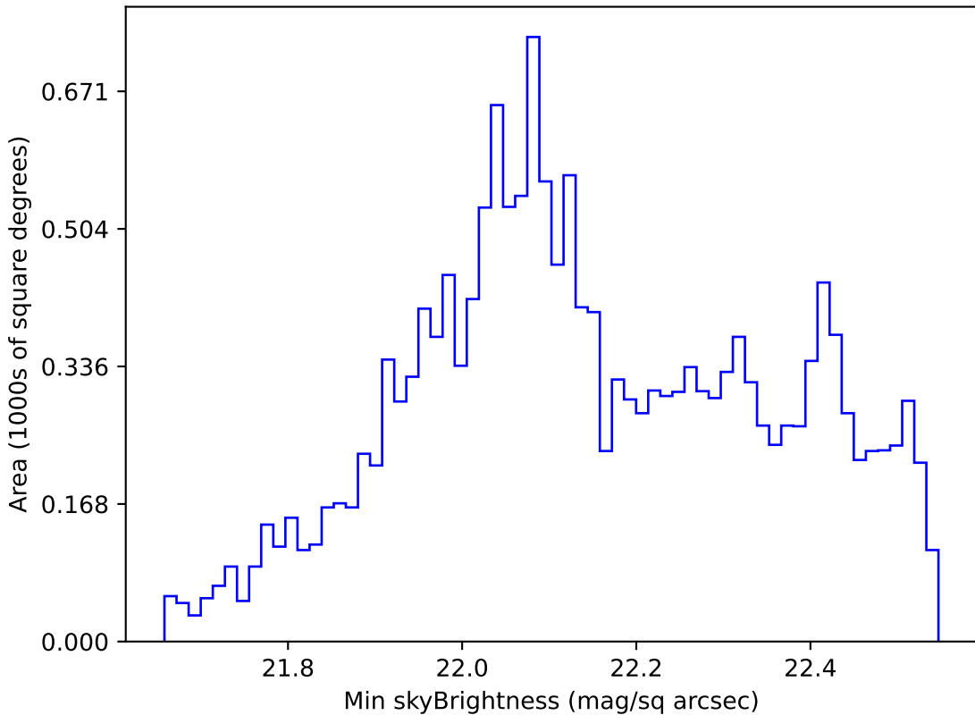
too_elab_r16_d2_gz_v3.4_10yrs WFD u band: Min skyBrightness
