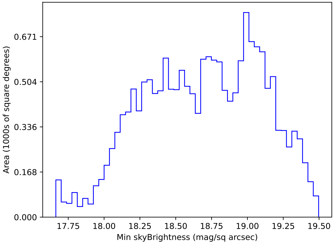
too_elab_r16_d2_gz_v3.4_10yrs WFD r band: Min skyBrightness
