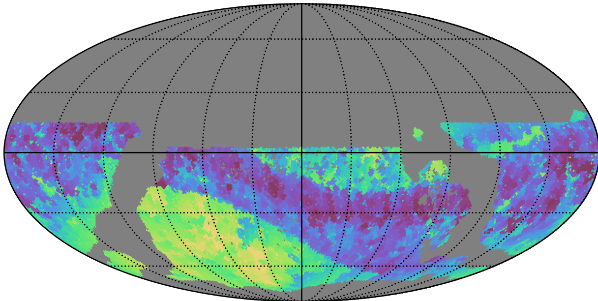
too_elab_r16_d2_gz_v3.4_10yrs WFD i band: Min skyBrightness
