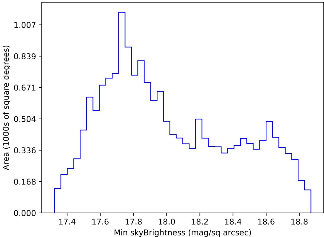
too_elab_r16_d2_gz_v3.4_10yrs WFD i band: Min skyBrightness
