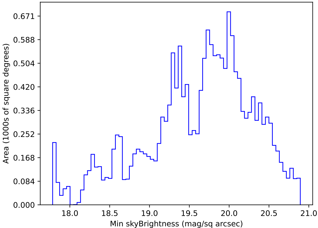
too_elab_r16_d2_gz_v3.4_10yrs WFD g band: Min skyBrightness
