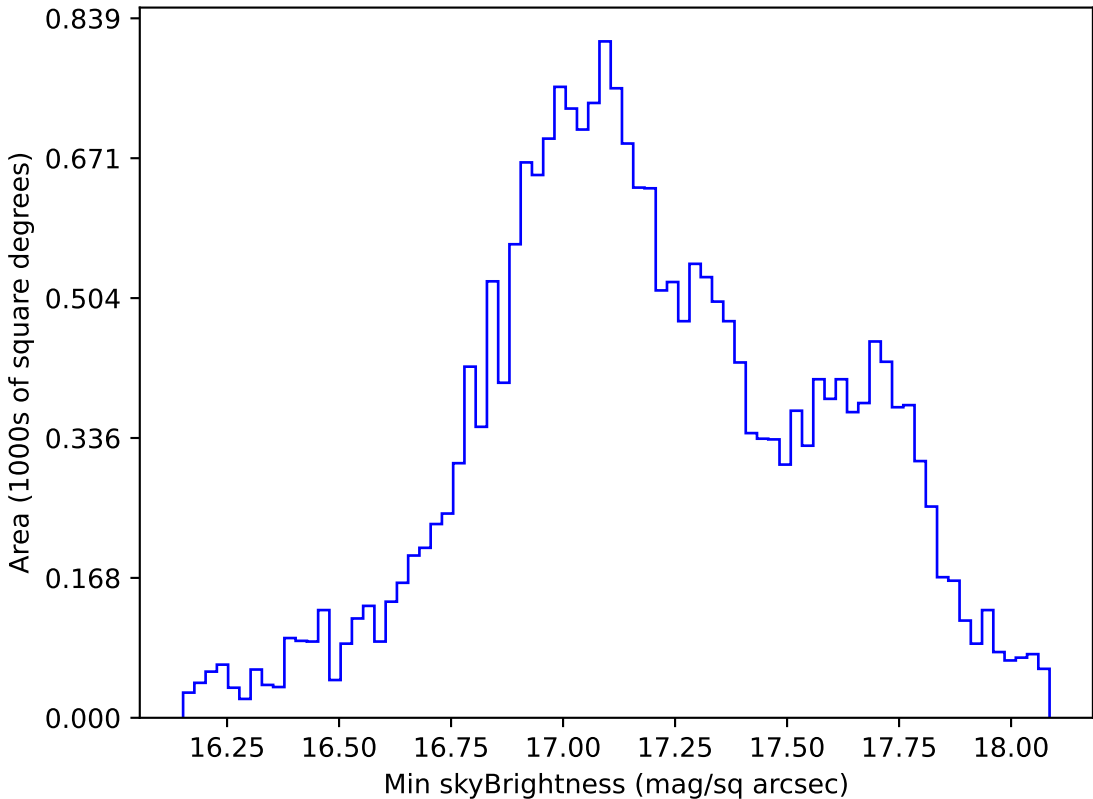
too_elab_r16_d2_gz_v3.4_10yrs All sky y band: Min skyBrightness
