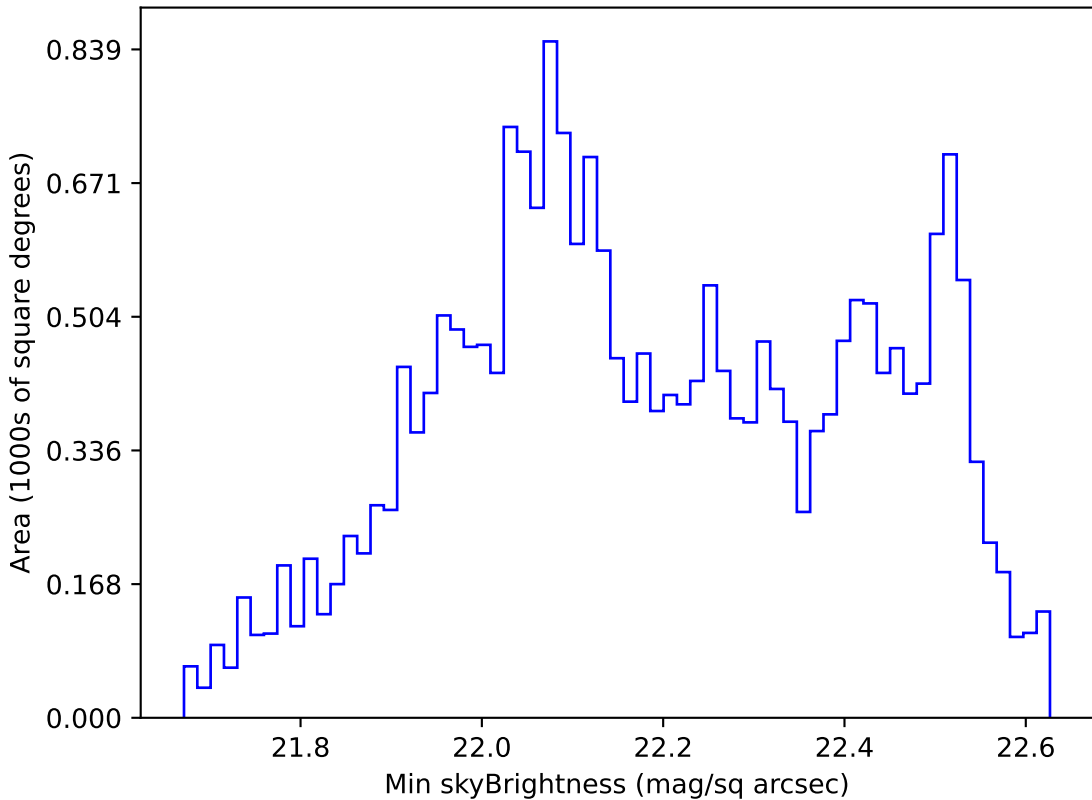
too_elab_r16_d2_gz_v3.4_10yrs All sky u band: Min skyBrightness
