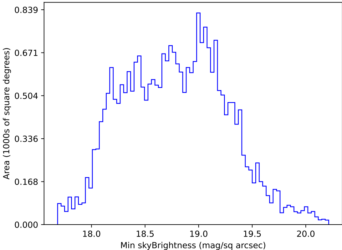
too_elab_r16_d2_gz_v3.4_10yrs All sky r band: Min skyBrightness
