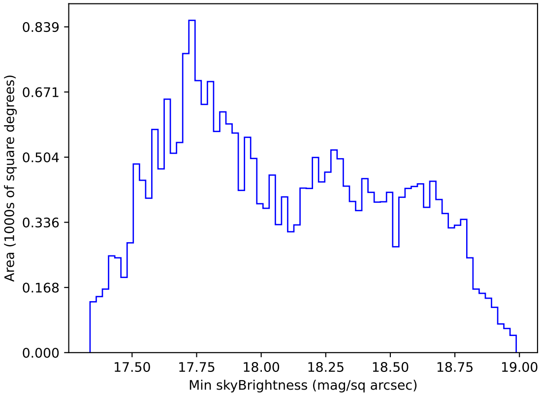
too_elab_r16_d2_gz_v3.4_10yrs All sky i band: Min skyBrightness
