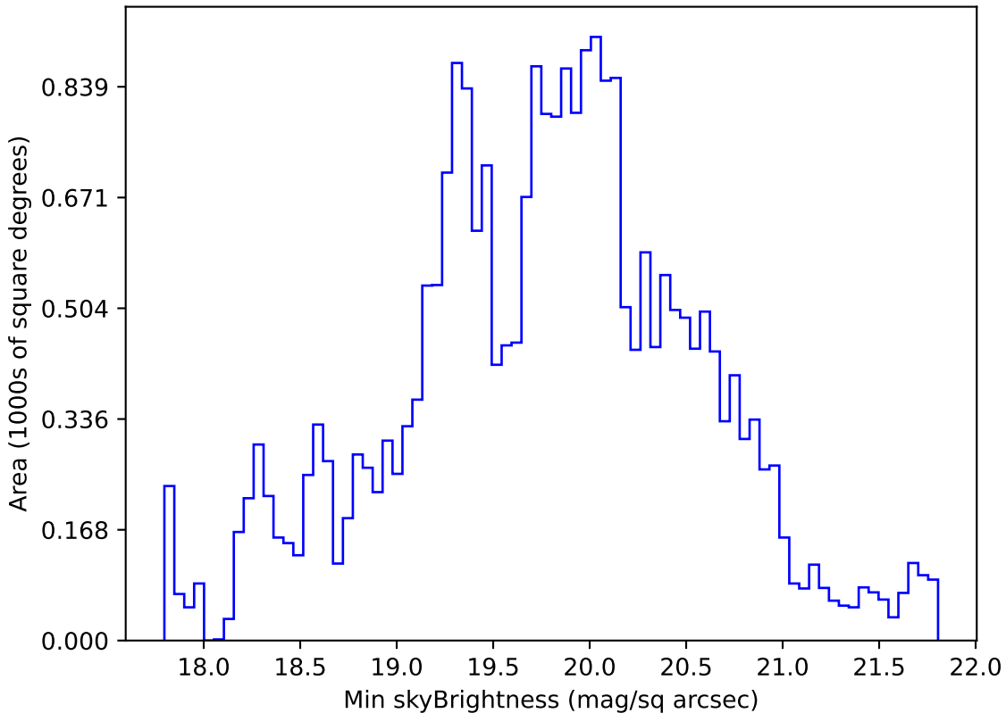
too_elab_r16_d2_gz_v3.4_10yrs All sky g band: Min skyBrightness
