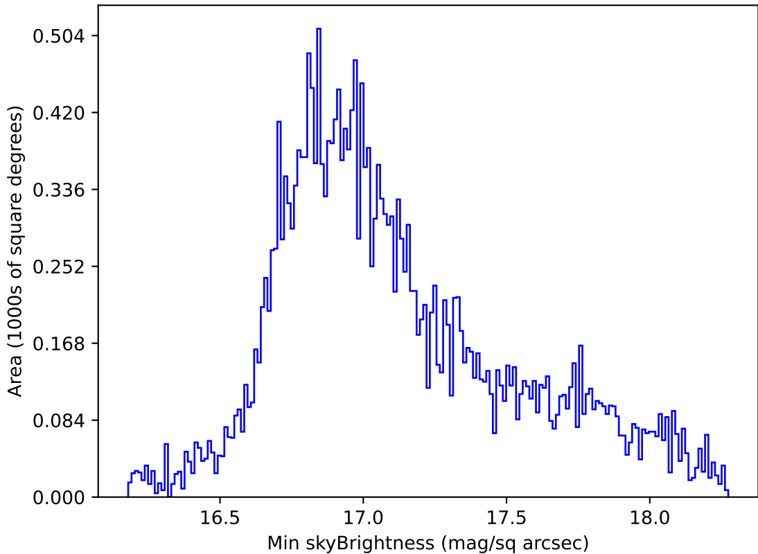
too_elab_r16_d2_gz_v3.4_10yrs All sky all bands: Min skyBrightness
