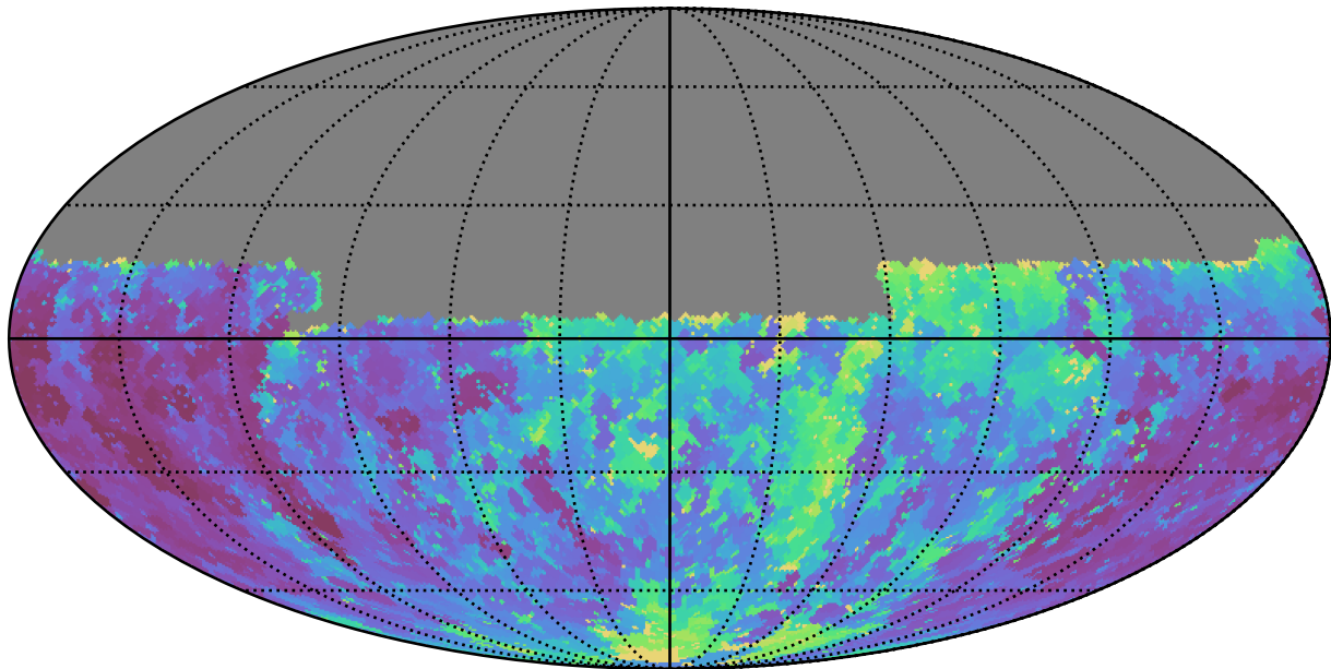
too_elab_r16_d2_gz_v3.4_10yrs Yr 1 u band: Min seeingGeom
