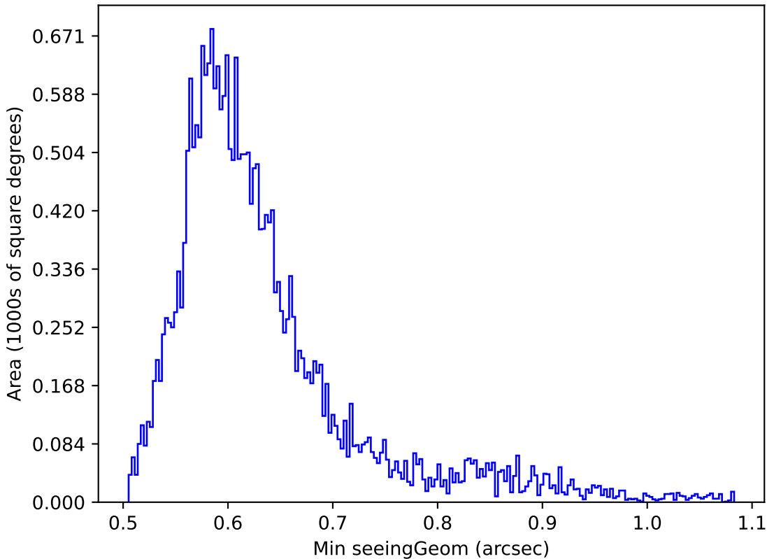
too_elab_r16_d2_gz_v3.4_10yrs Yr 1 i band: Min seeingGeom
