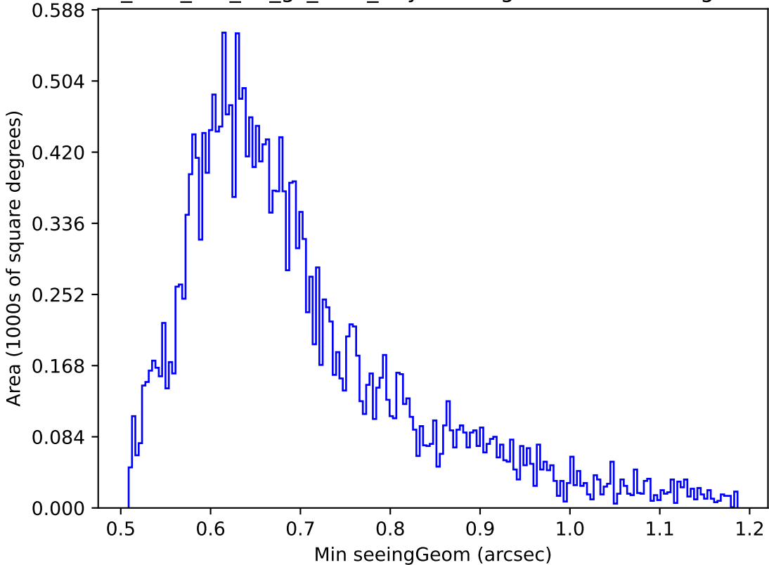
too_elab_r16_d2_gz_v3.4_10yrs Yr 1 g band: Min seeingGeom
