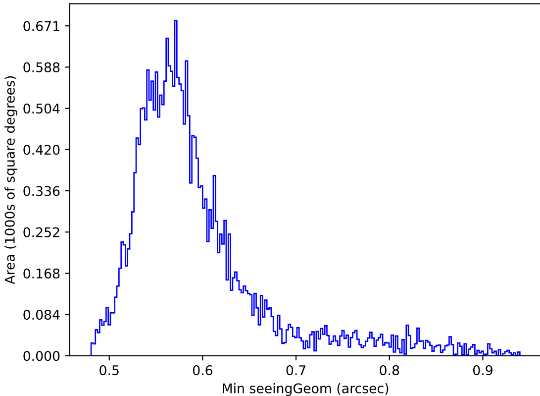
too_elab_r16_d2_gz_v3.4_10yrs Yr 1 all bands: Min seeingGeom
