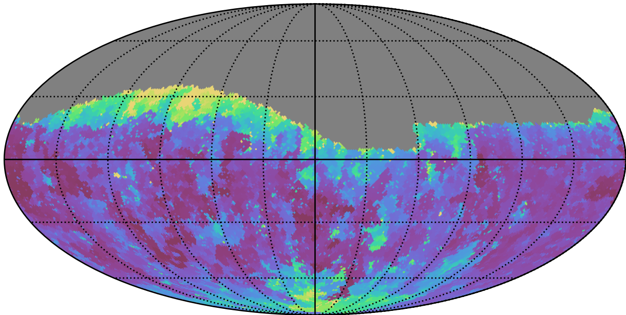
too_elab_r16_d2_gz_v3.4_10yrs Yr 1 g band: Min seeingEff
