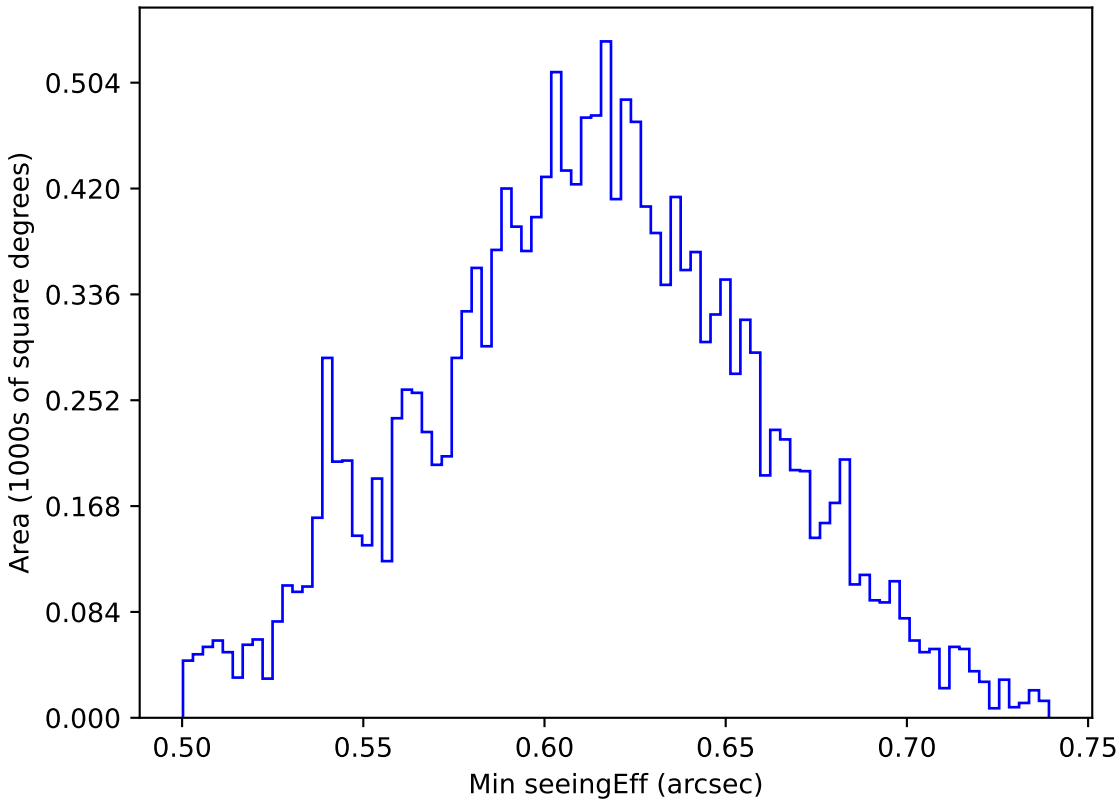
too_elab_r16_d2_gz_v3.4_10yrs WFD r band: Min seeingEff
