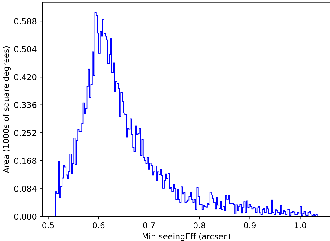
too_elab_r16_d2_gz_v3.4_10yrs All sky z band: Min seeingEff
