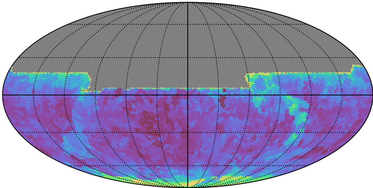
too_elab_r16_d2_gz_v3.4_10yrs All sky y band: Min seeingEff
