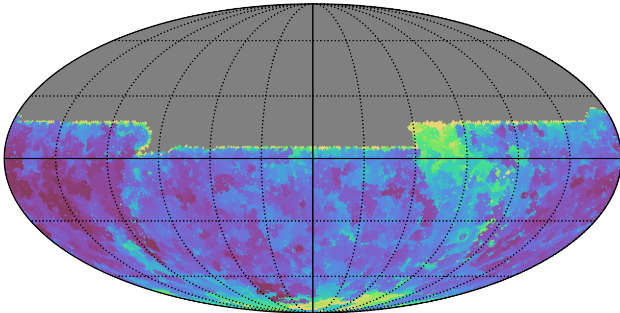
too_elab_r16_d2_gz_v3.4_10yrs All sky u band: Min seeingEff
