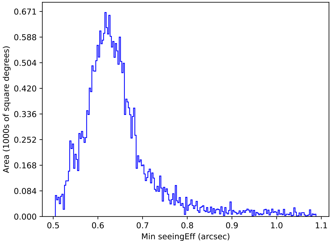
too_elab_r16_d2_gz_v3.4_10yrs All sky r band: Min seeingEff
