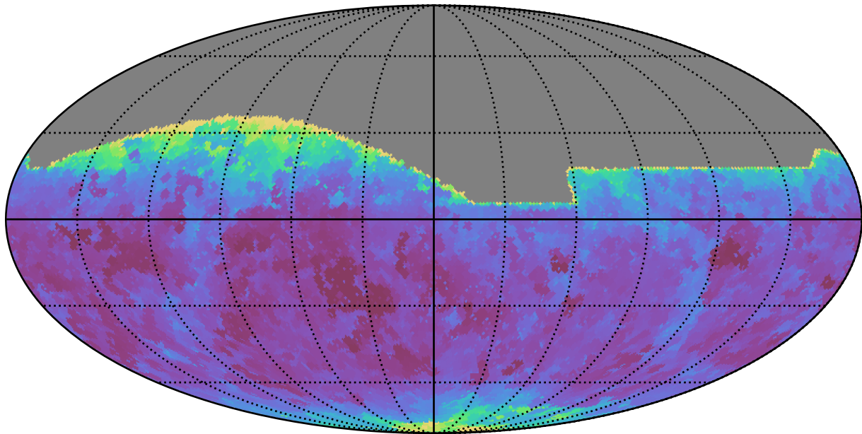
too_elab_r16_d2_gz_v3.4_10yrs All sky i band: Min seeingEff
