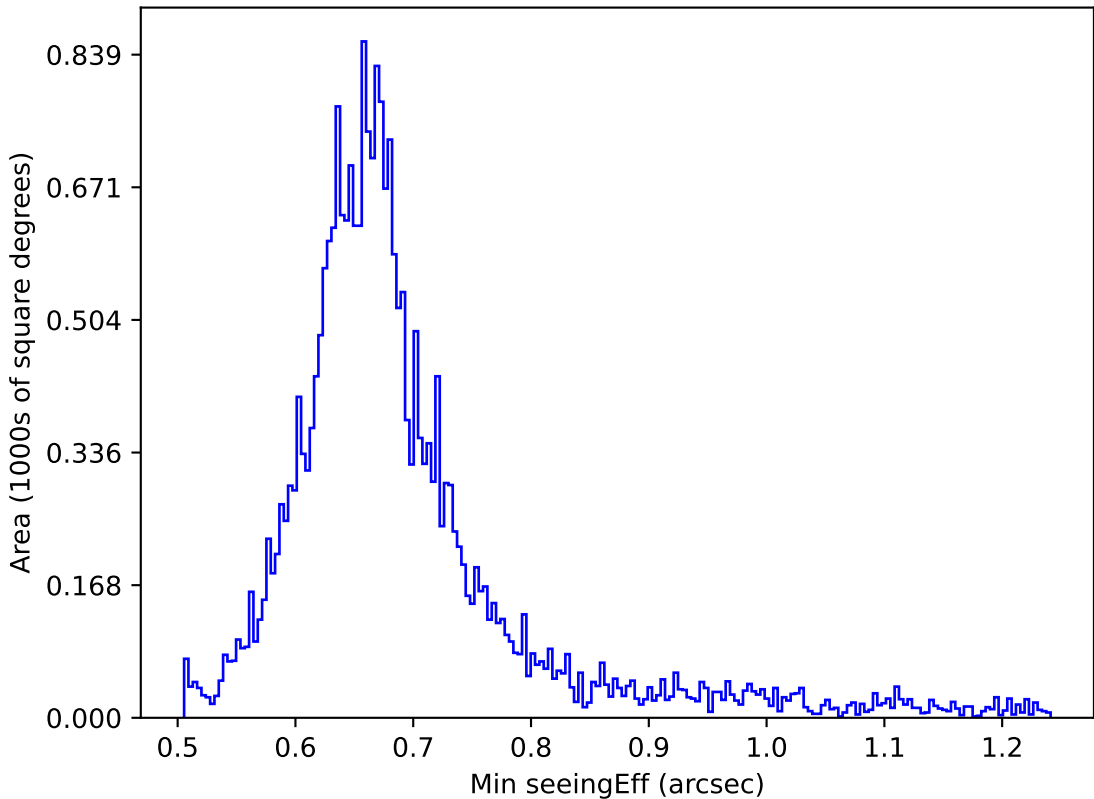
too_elab_r16_d2_gz_v3.4_10yrs All sky g band: Min seeingEff
