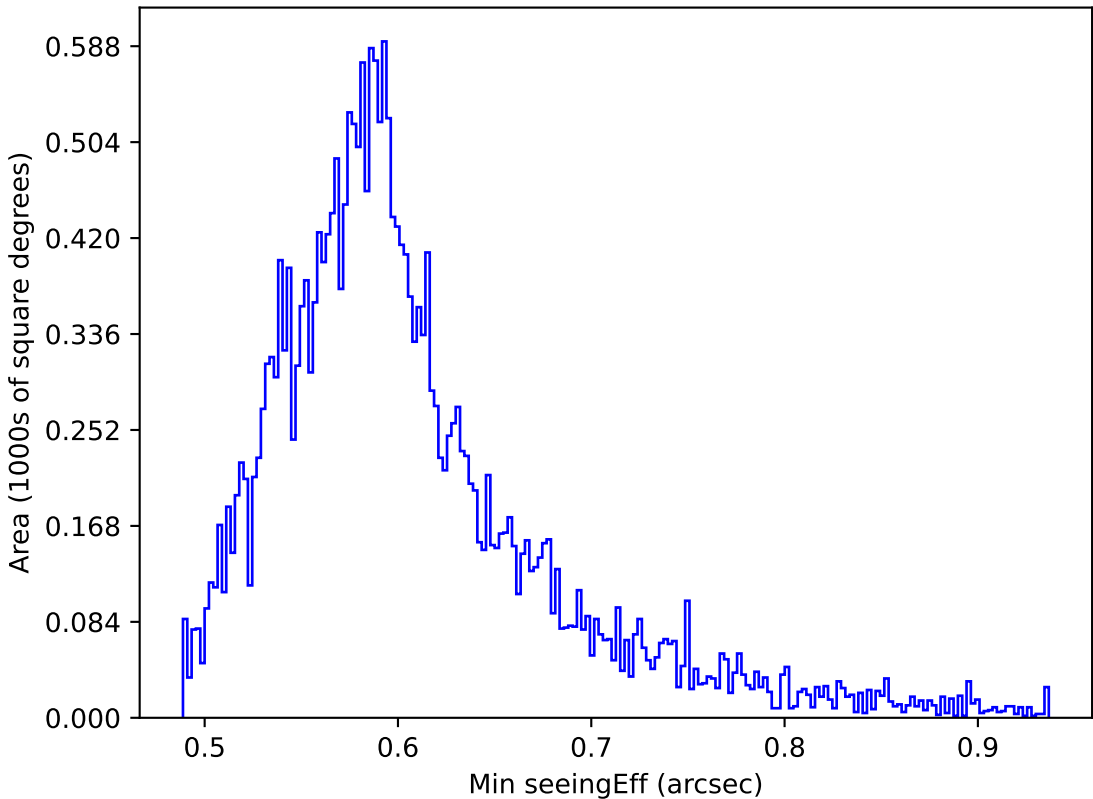
too_elab_r16_d2_gz_v3.4_10yrs All sky all bands: Min seeingEff
