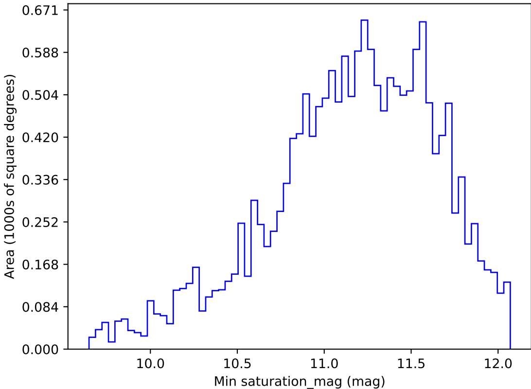
too_elab_r16_d2_gz_v3.4_10yrs WFD y band: Min saturation_mag
