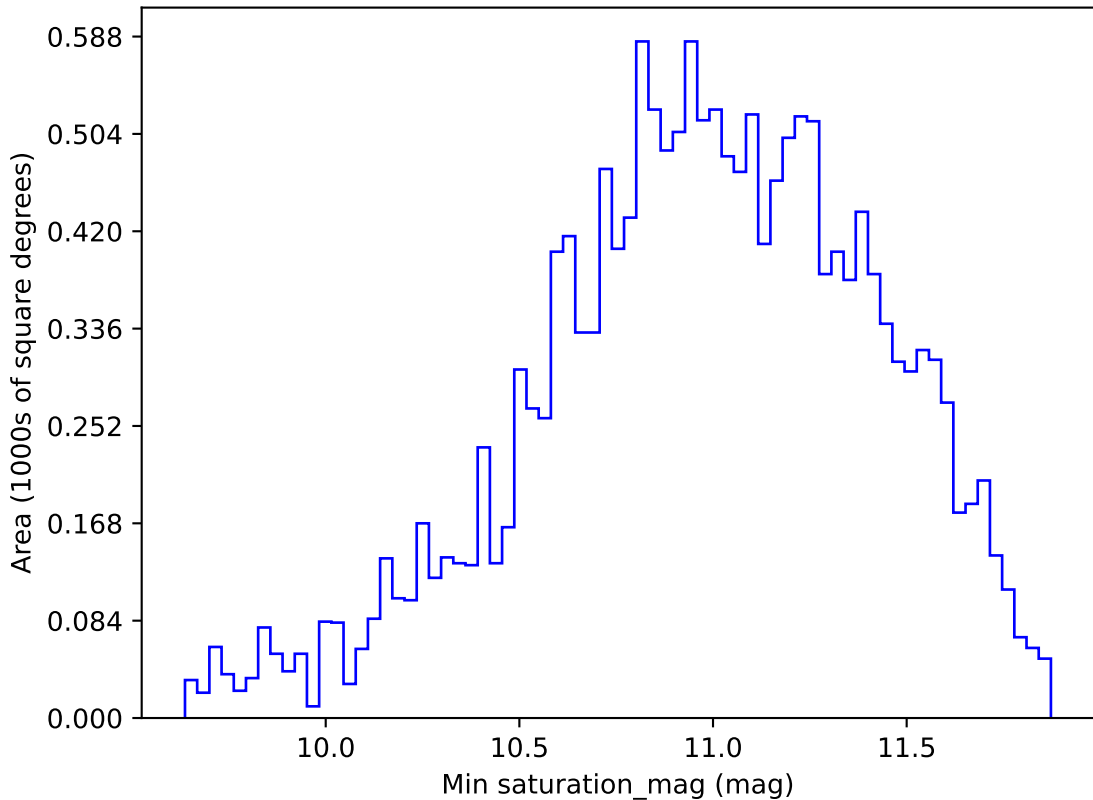
too_elab_r16_d2_gz_v3.4_10yrs WFD all bands: Min saturation_mag
