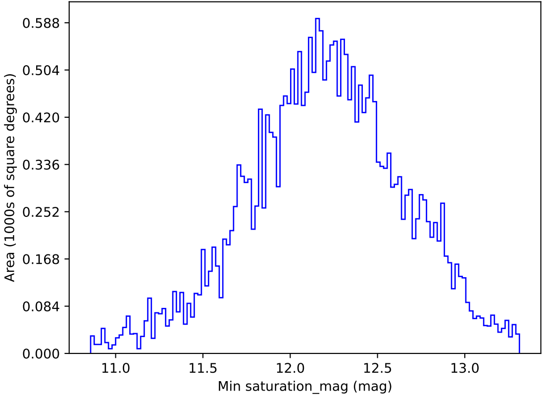
too_elab_r16_d2_gz_v3.4_10yrs All sky z band: Min saturation_mag
