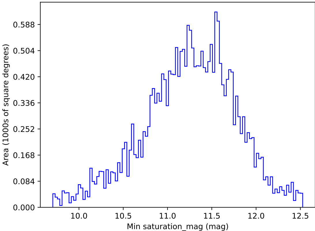
too_elab_r16_d2_gz_v3.4_10yrs All sky y band: Min saturation_mag
